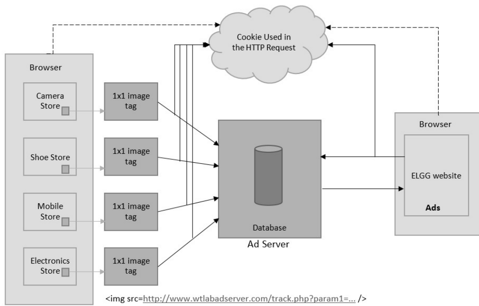
Figure 4: High level architecture diagram of web tracking
