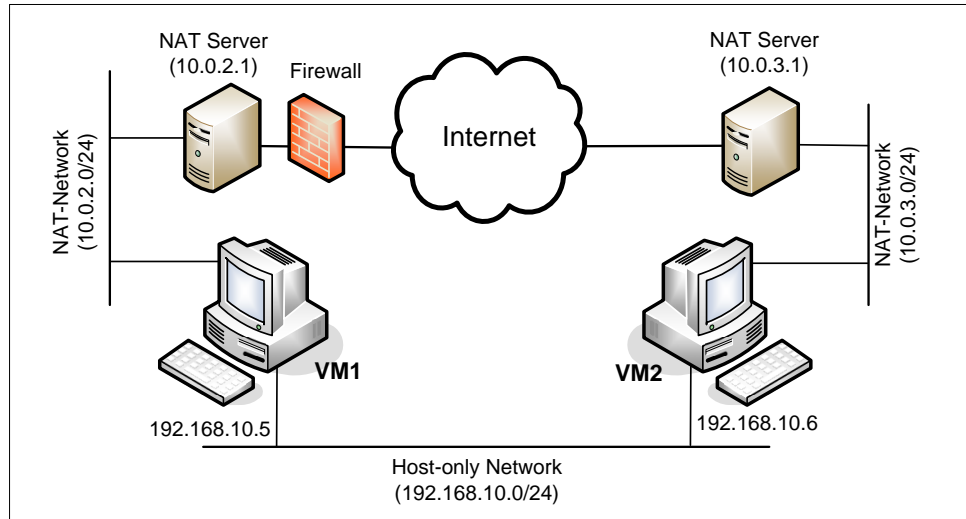
Figure 1: Lab Environment Setup
