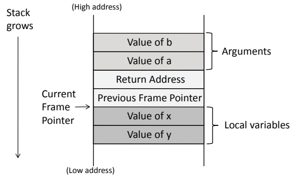
Figure 4.2: Layout for a function's stack frame
